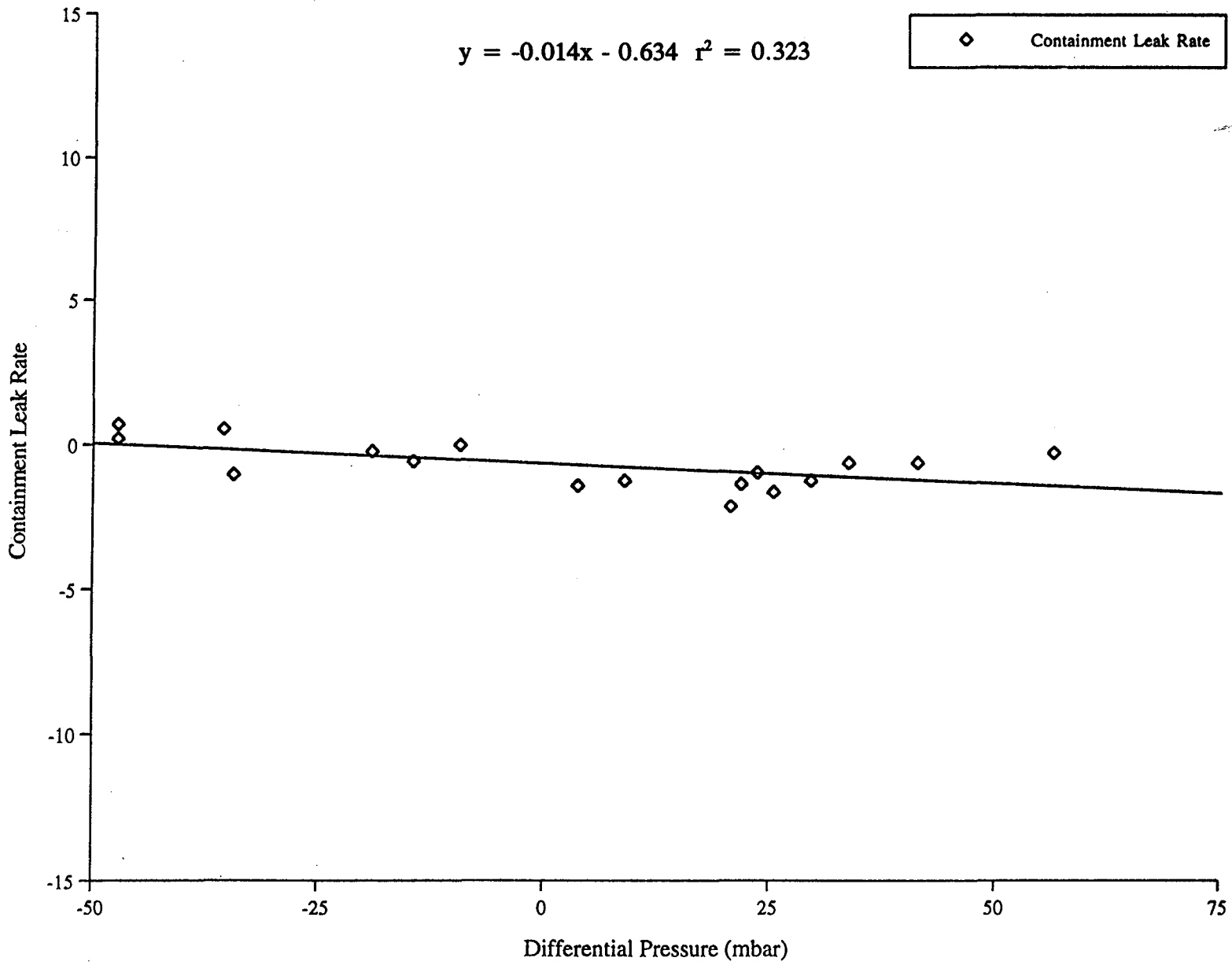
Figure C-2. Containment Leak Rate
