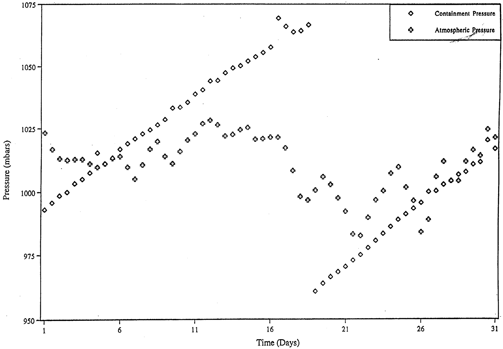
Figure C-1. Typical Containment Air Pressure Cycle
