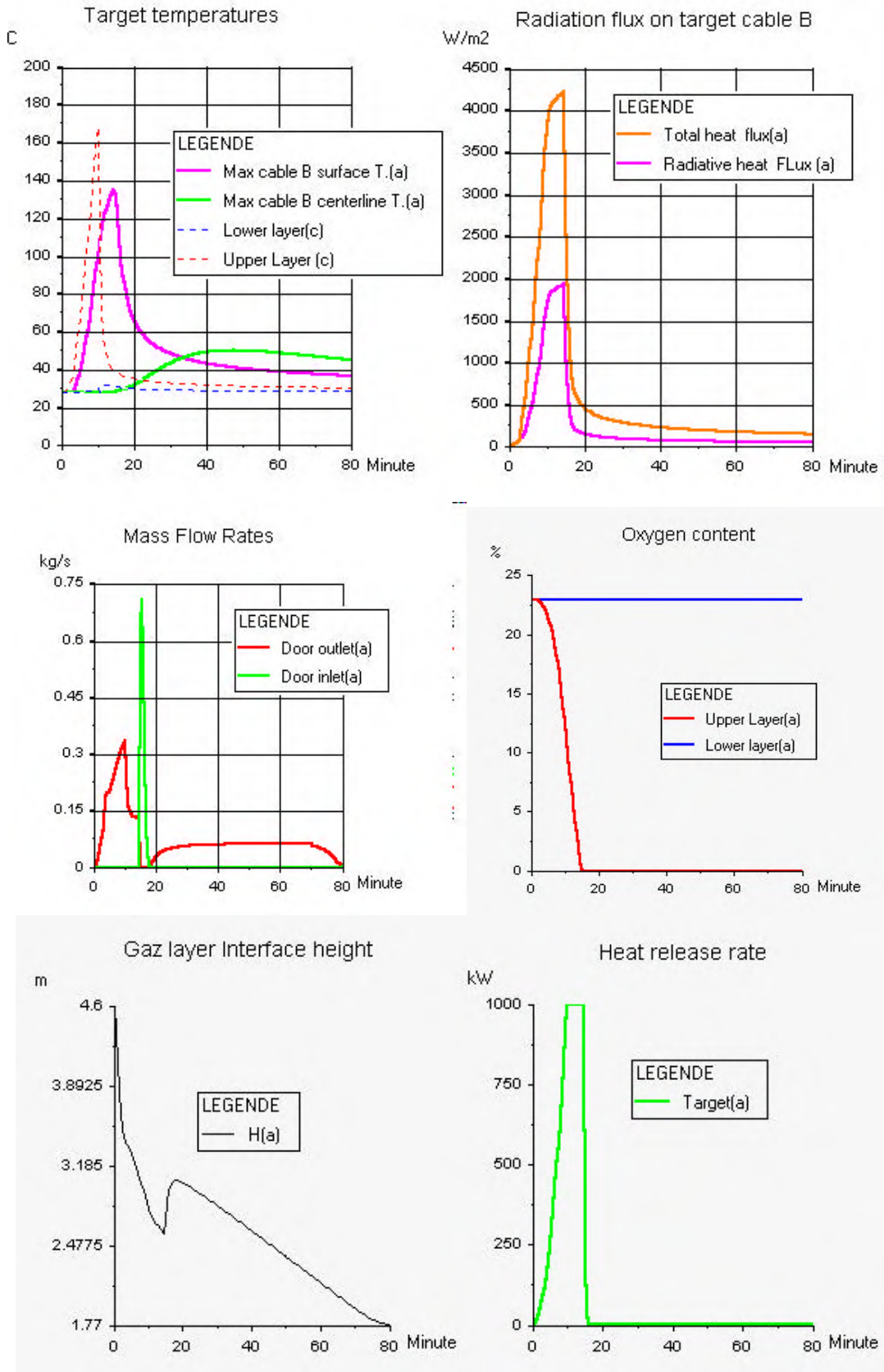
Figure 7: Part II Base case (LOL=0%)
