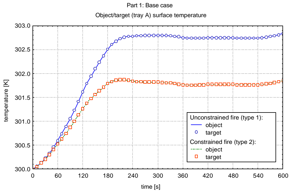
Figure 2.6 Surface temperature of tray A (base case)
