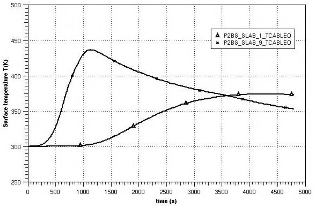
Figure 6-6 Surface and inner temperature of the target
