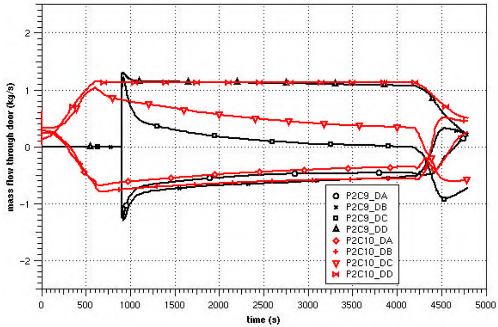
Figure 6-26 Mass flow rate through door (case 9 and 10)
