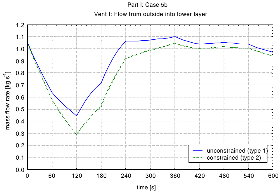
Figure 2.21 Mass flow rate through air inlet (outside- lower layer)
