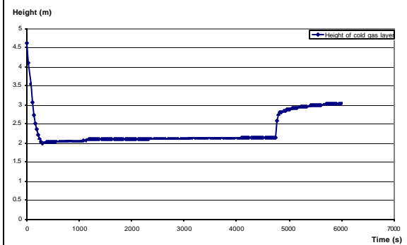
Figure 2 : Height of cold gas layer
