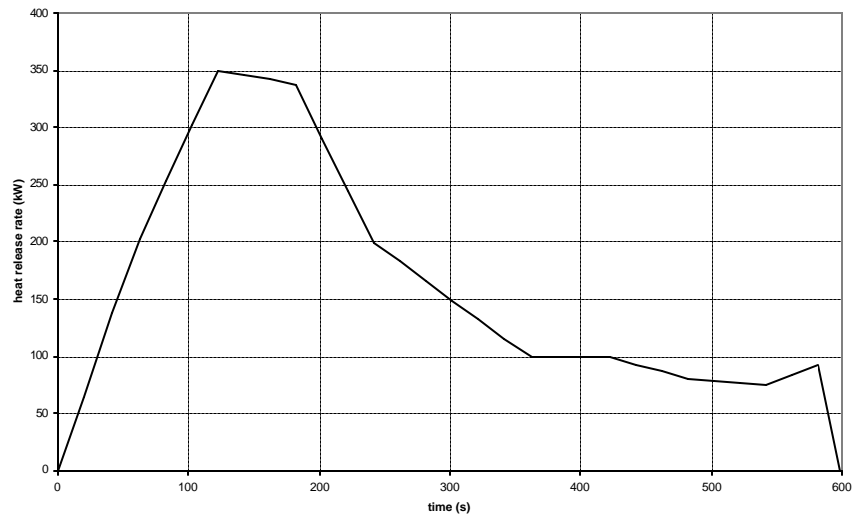
Figure 5: Heat release rate of the fire.
