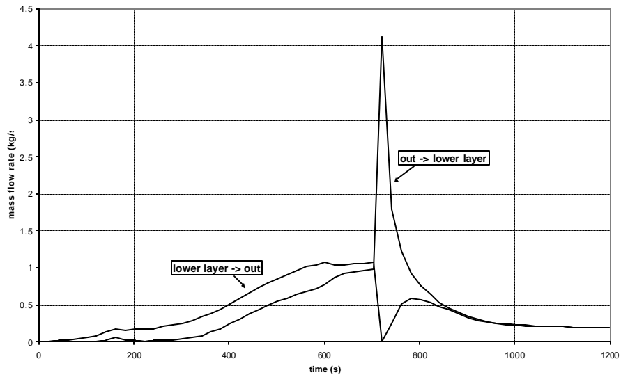
Figure 46: Flow rate through the door.
