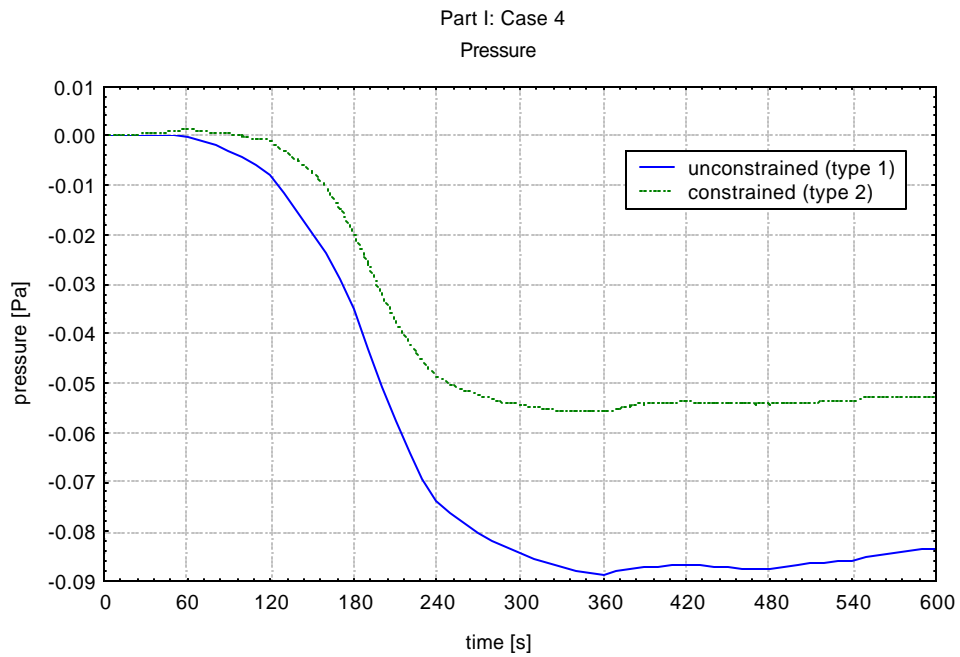
Figure 2.25 Pressure (case 4)
