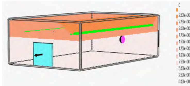
figure 10 : smoke filling at t=600s in case 9
