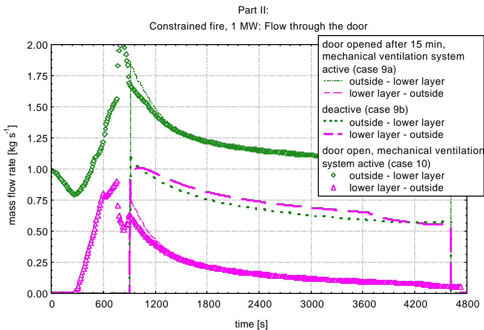
Figure 3.19 Effect of mechanical ventilation system: Mass flow rate through the door
