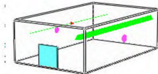
Part 2: redundant tray B exposed to a trash bag tray A cable fire (13 cases studied)
