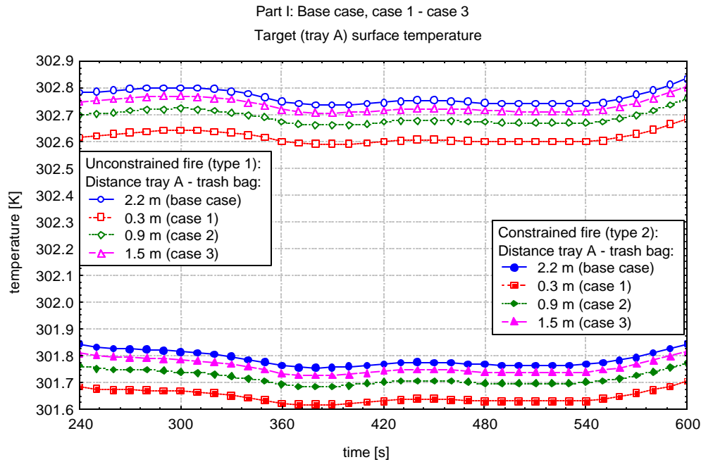
Figure 2.7 Surface temperature of tray A, unconstrained fire (base case, cases 1- 3)
