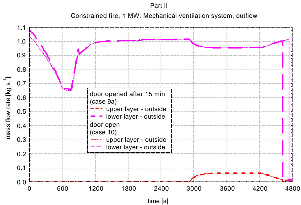
Figure 3.21 Effect of door opening: Mass flow rate through duct system (outflow)
