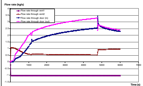
Figure 6 : Flow rate through vents and door
