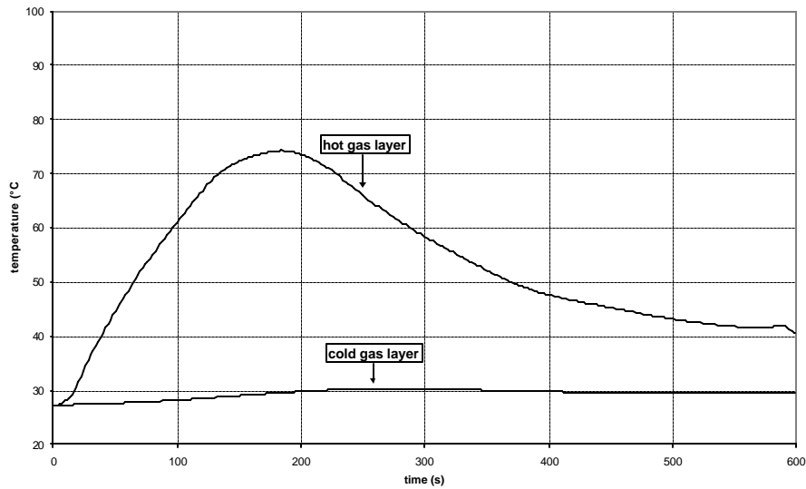
Figure 6: Room temperature.
