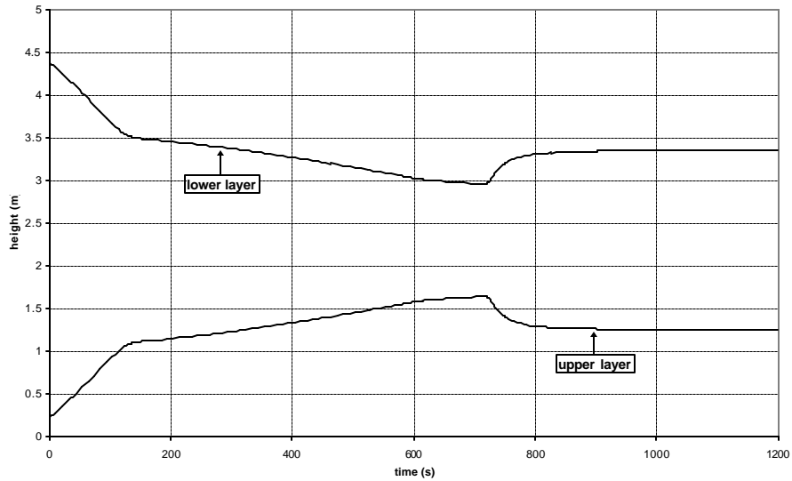
Figure 25: Depth of upper and lower layers.
