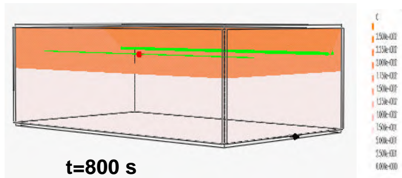
figure 6: smoke filling in part II base case at t=800s
