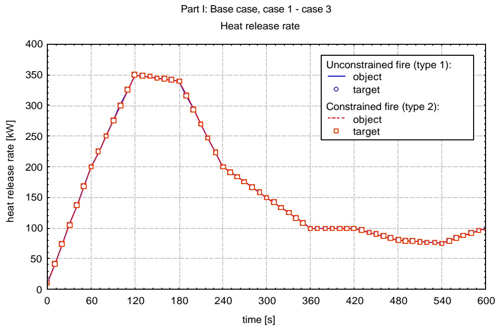
Figure 2.4 Heat release rate (base case, cases 1 - 3)
