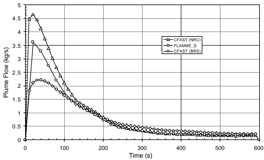
Figure 3 Plume Flow (Part I, Base Case)
