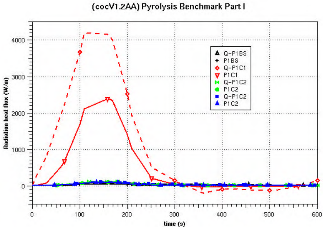
Figure 5-11 Radiation heat flux on the target
