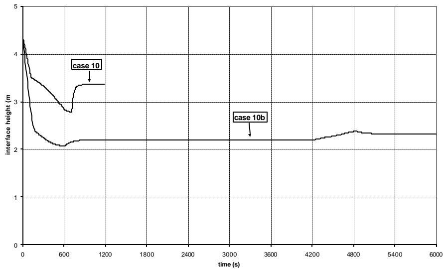
Figure 31: Interface height in the room.
