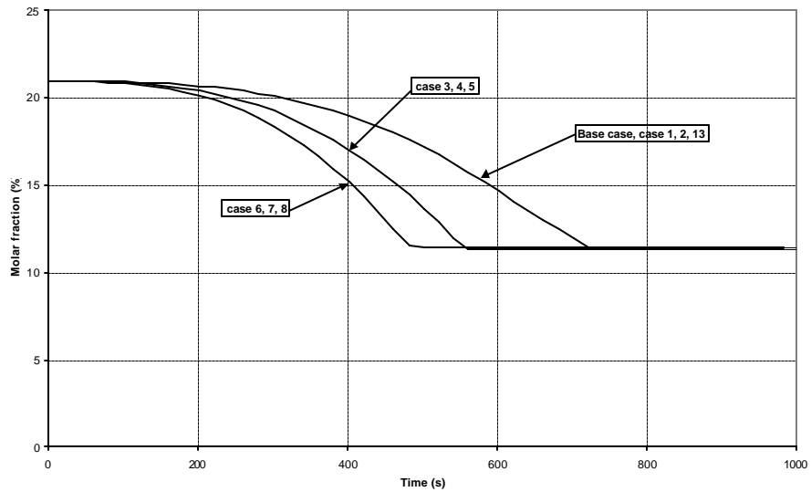
Figure 20 : Oxygen molar fraction in the upper layer
