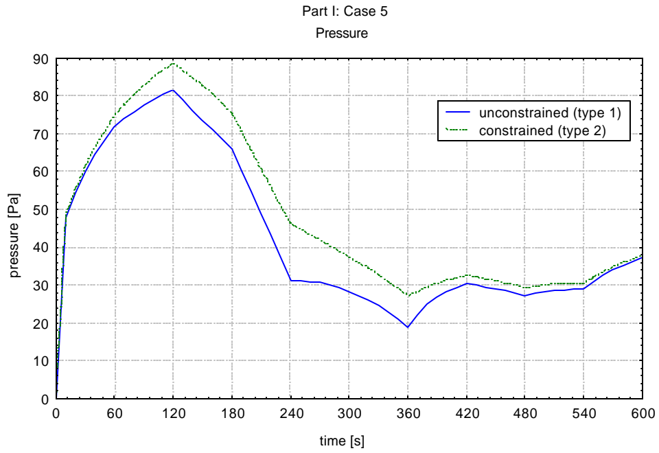
Figure 2.26 Pressure (case 5)
