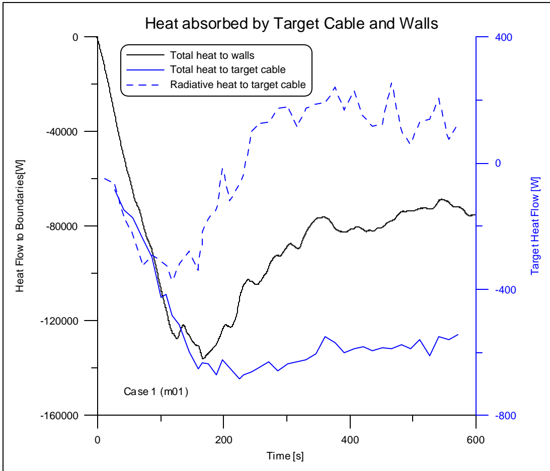
Fig. 11 Heat fluxes for case 1
