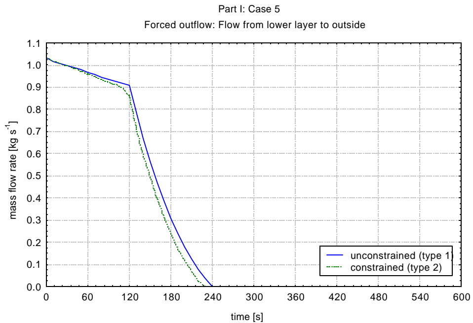
Figure 2.22 Mass flow rate of fan (lower layer- outside)
