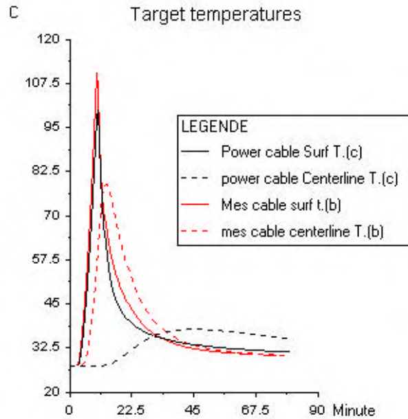
figure 11: effect of cable structure and elevation
