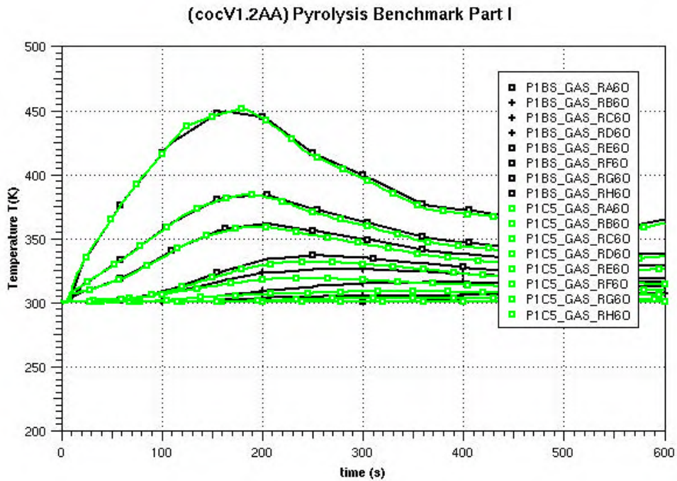
Figure 5-16 Comparison of temperatures (ventilation system)
