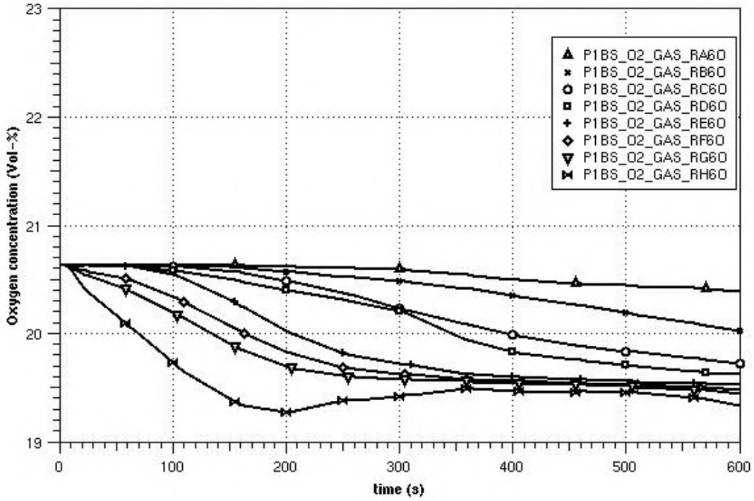
Figure 5-3 Oxygen concentration in the room centre
