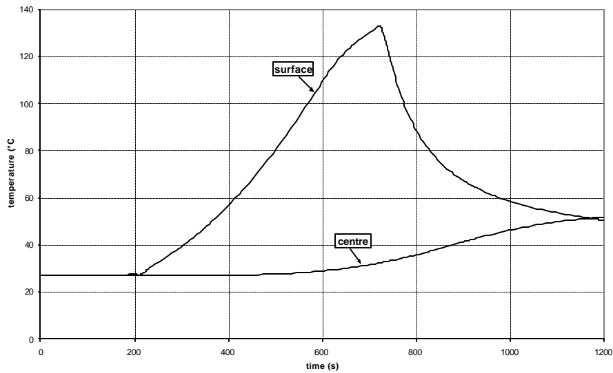
Figure 28: Cable temperature (target).
