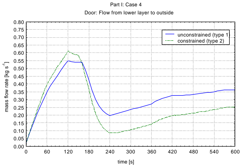
Figure 2.19 Mass flow rate through the opened door (lower layer - outside)
