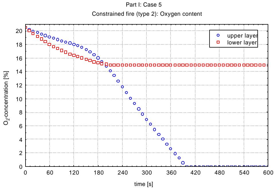
Figure 2.9 Oxygen content (case 5)
