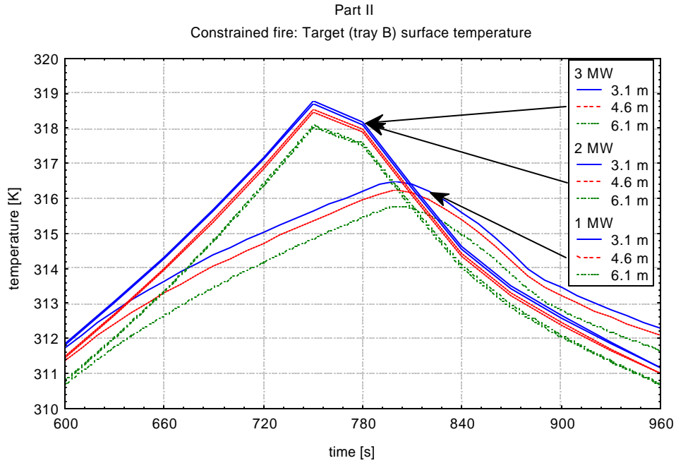
Figure 3.26 Effect of heat release rate and distance: Target (tray B) surface temperature
