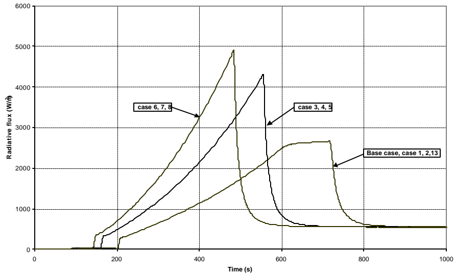
Figure 42 : Incident radiant flux on the target
