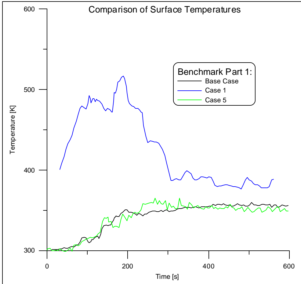
Fig. 15 Comparison of surface temperatures for benchmark part 1
