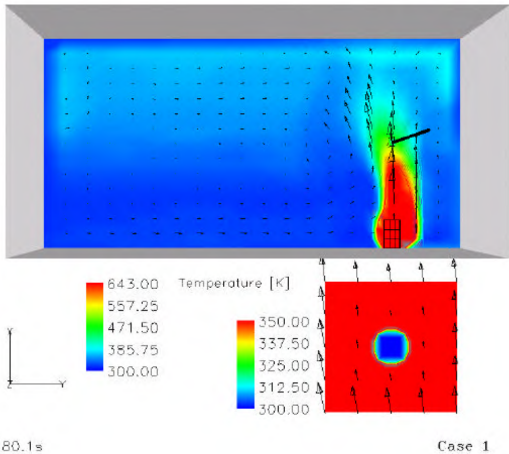
Fig. 10 Flow field and temperature distribution in the room for case 1
