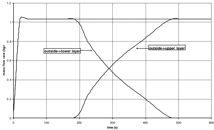
Figure 37: Mass flow rate through the supply vent.
