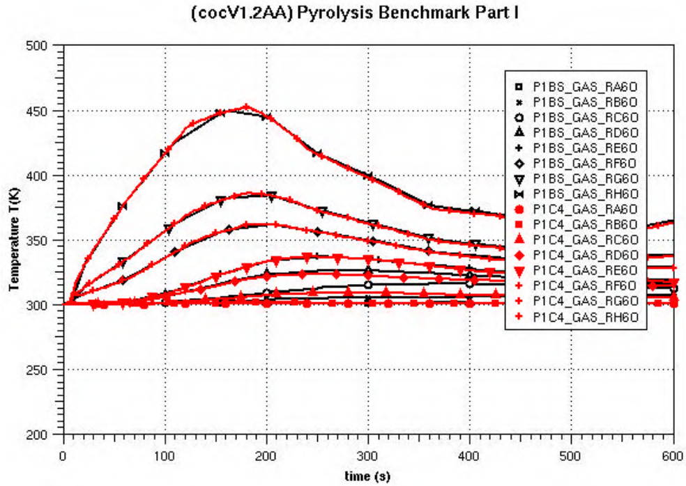
Figure 5-15 Comparison of temperatures (open doors)
