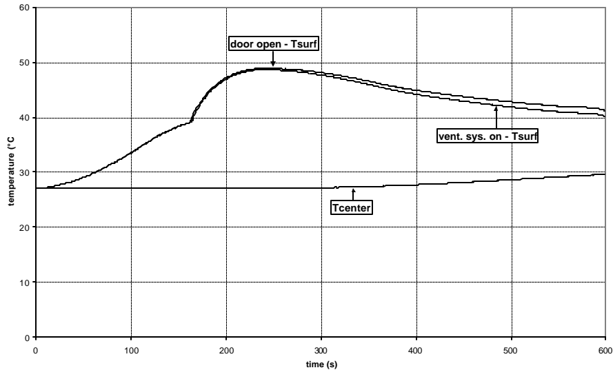
Figure 12: Cable temperature.
