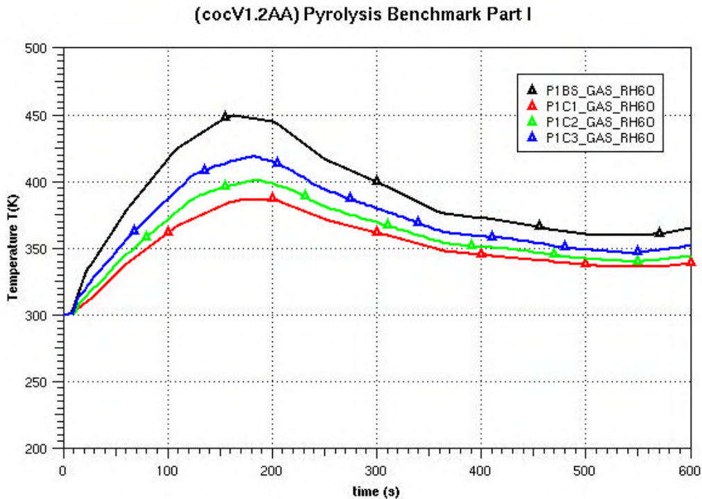
Figure 5-8 Atmospheric temperatures in the centre below the ceiling (RH60)
