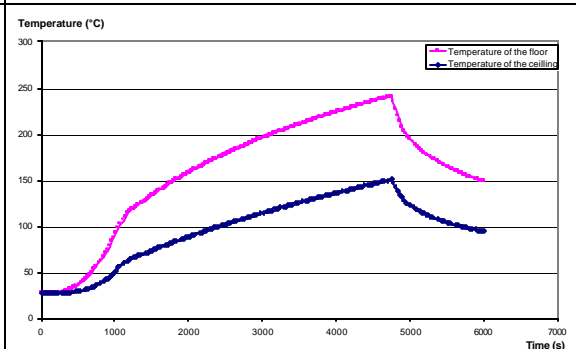
Figure 8 : Floor and ceiling temperature
