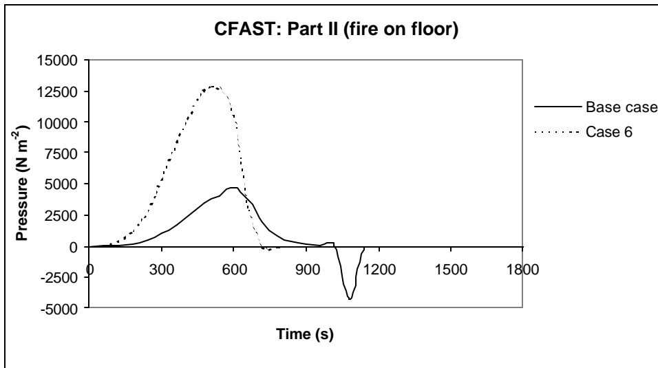
Figure 19 CFAST predictions of pressure in Part II
