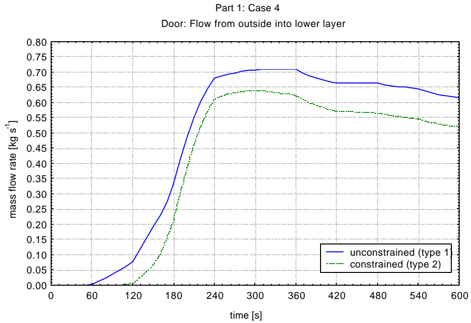
Figure 2.18 Mass flow rate through the opened door (outside - lower layer)
