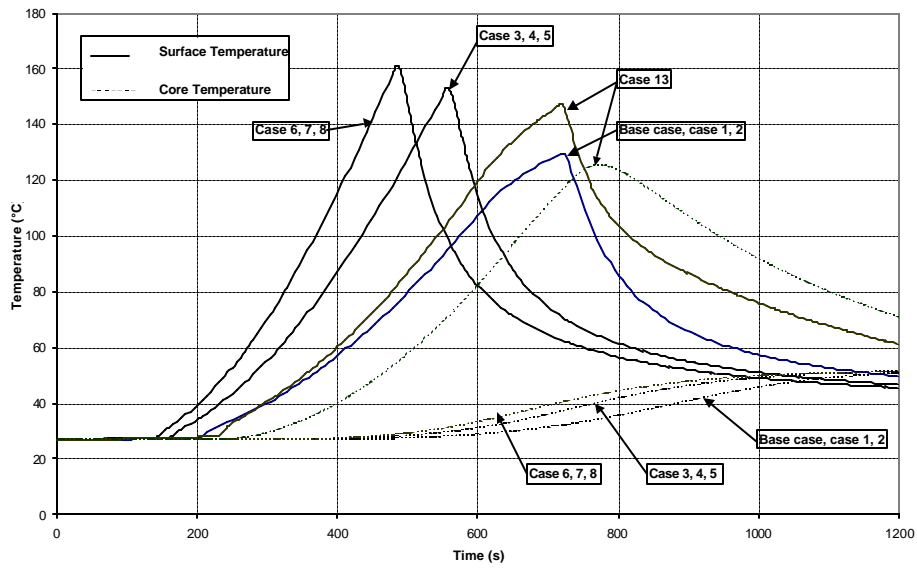
Figure 29 Effect of Cable Structure (from Bouton (Appendix A))
