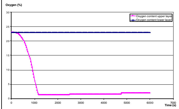
Figure 4 : Oxygen concentration
