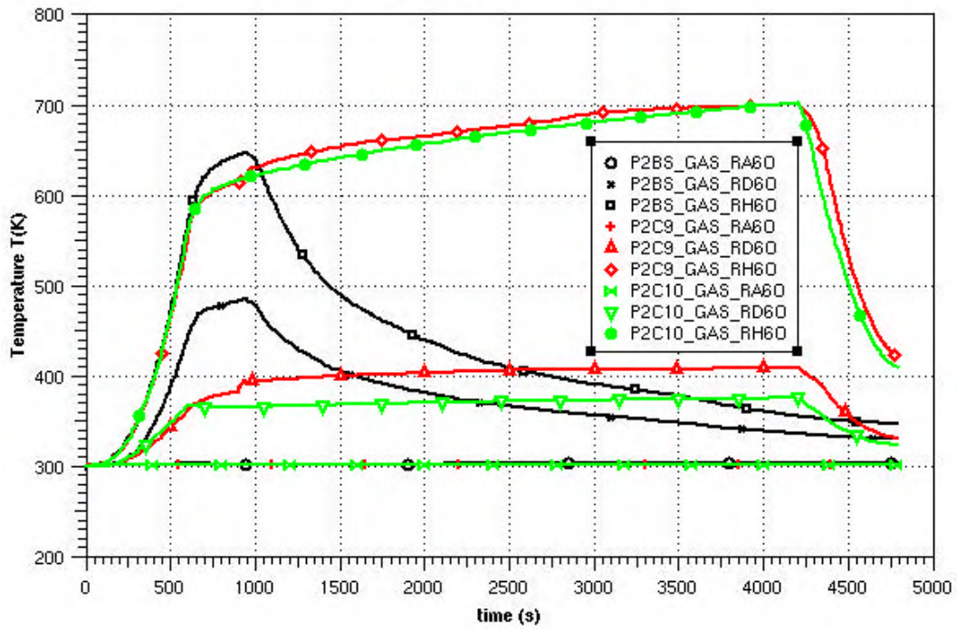
(cocV1.2AA) Pyrolysis Benchmark Part II
