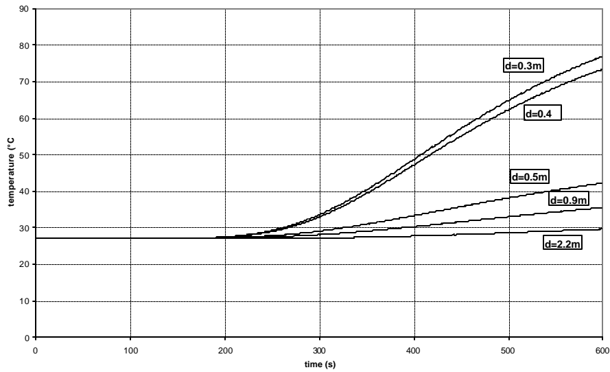
Figure 10: Temperature inside the cable.
