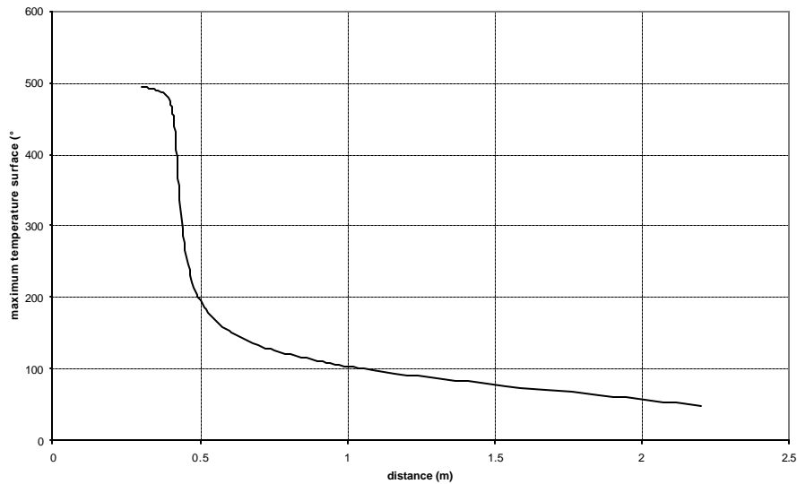
Figure 9: Maximum temperature "surface" of the cable.
