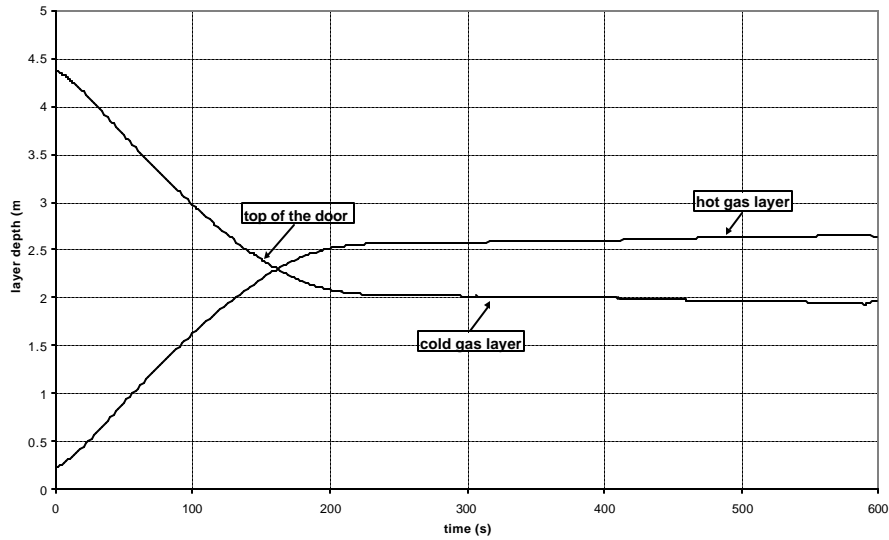
Figure 35: Depth of the upper and lower layers.
