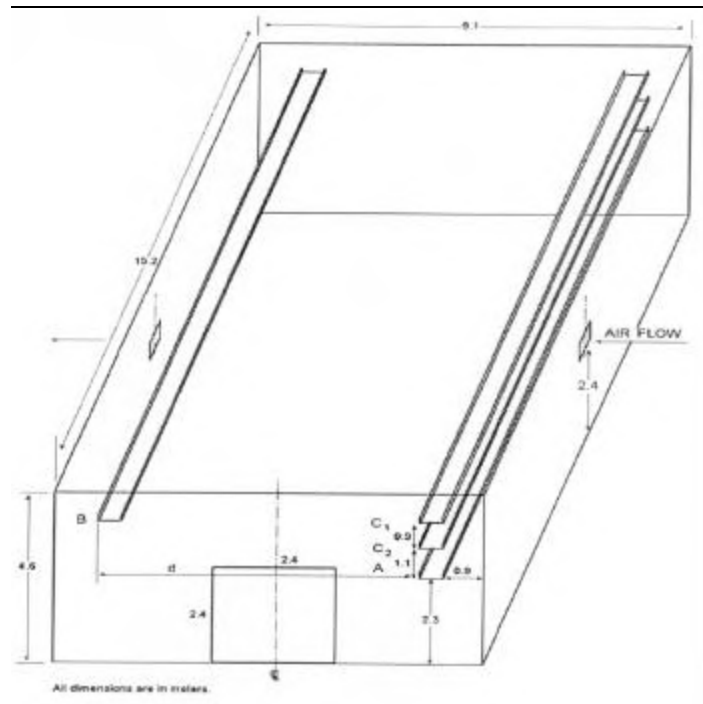
Figure 1: Geometry.
