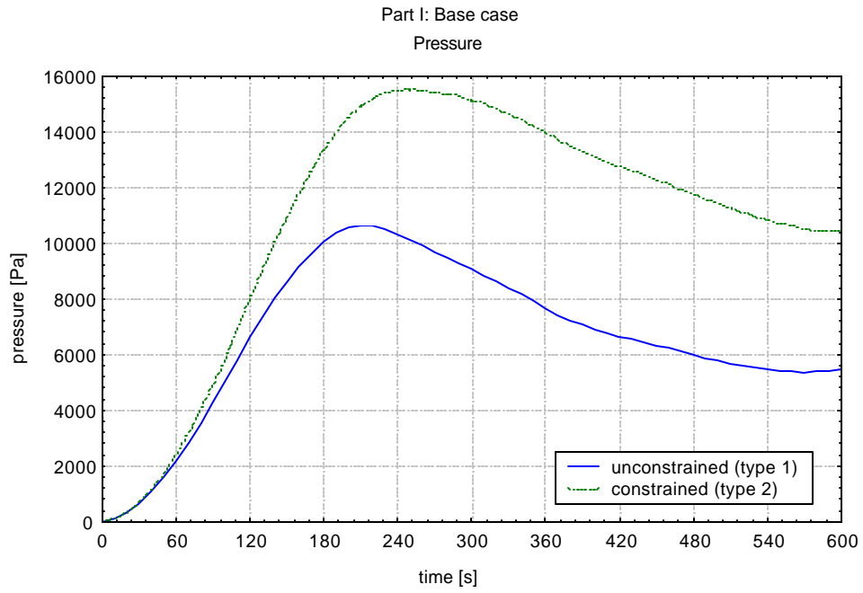
Figure 2.24 Pressure (base case)
