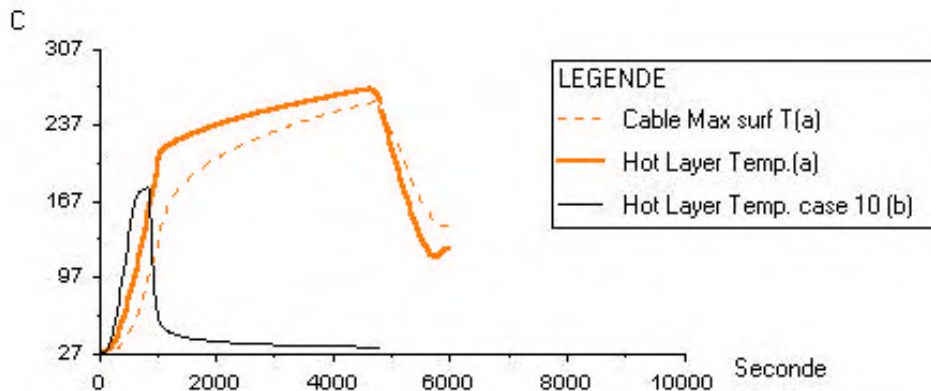
Part II: Effect of a lower location of cable fire : 1 m above floor in case 10
