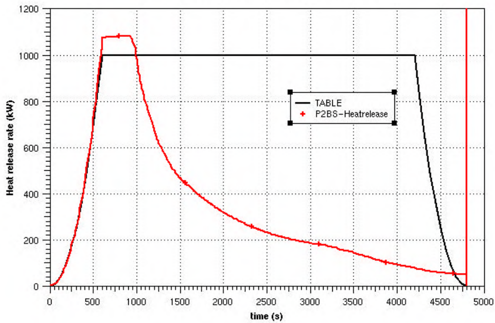
Figure 6-2 Heat release
