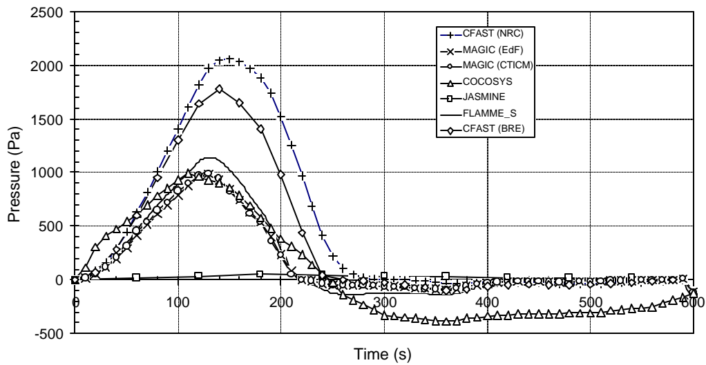
Figure 6 Pressure Development (Part I, Base Case)
