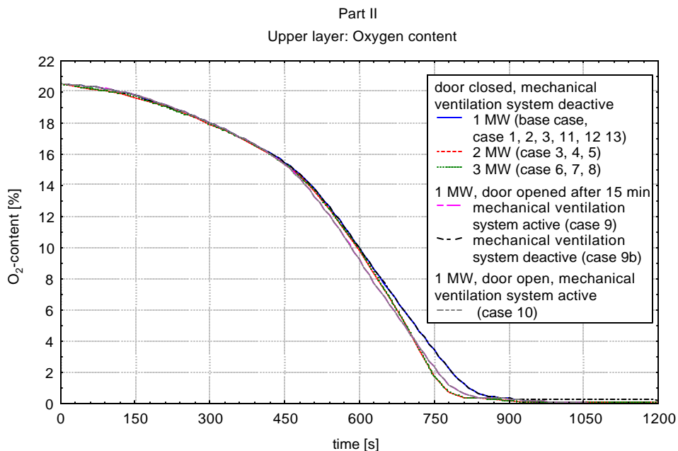
Figure 3.17 Effect of heat release rate and ventilation condition: Oxygen in the upper layer
