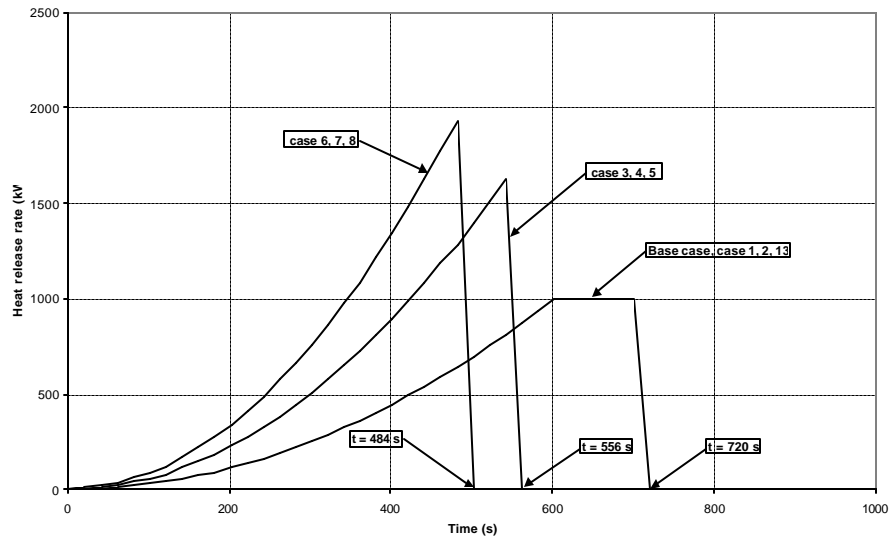
Figure 19 : Actual heat release rate
