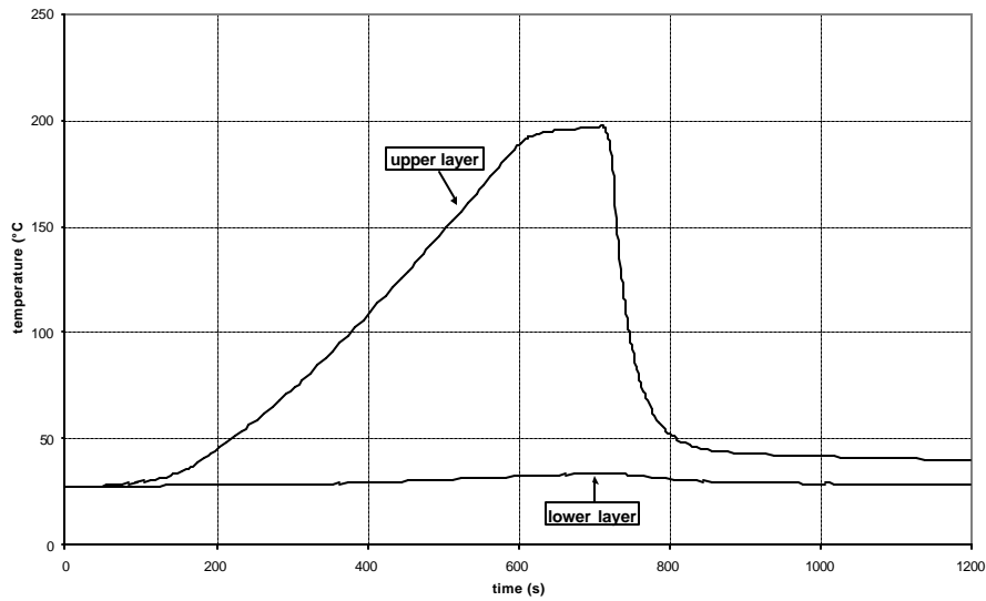
Figure 27: Room temperatures.
